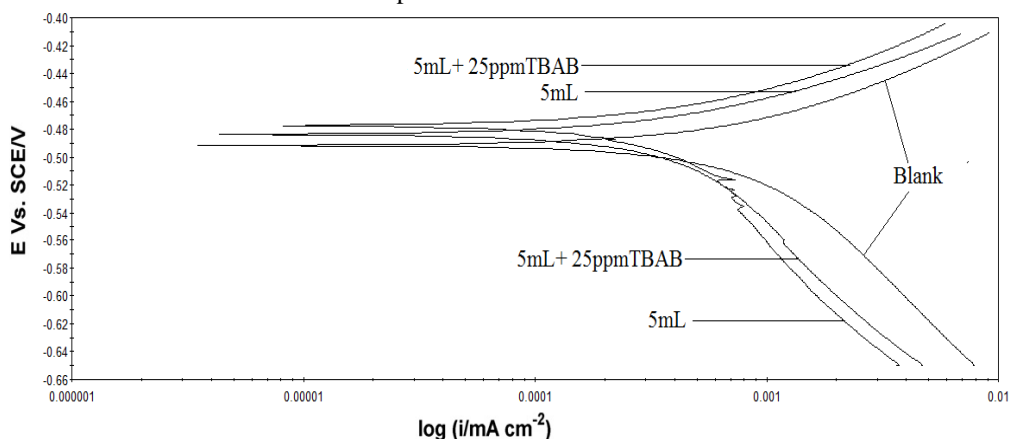
Fig 2. Potentiodynamic polarization curves of mild steel immersed in 0.5M H 2 SO 4 solution in the absence and presence of inhibitors
